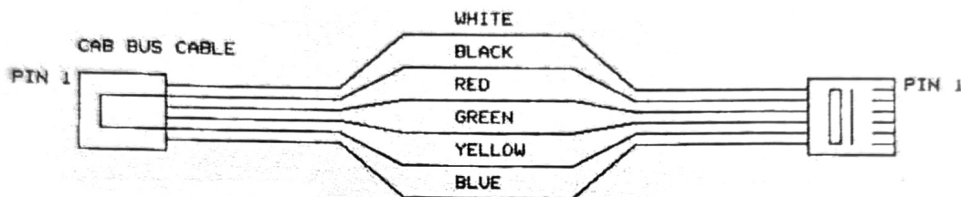
GENERAL RJ TYPE CABLE ORIENTATION
